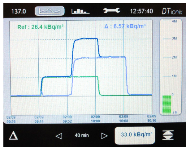
Injection of 1 MBq/m 3 (27 \mu Ci/m 3 ) of tritium HT then 2 MBq/m 3 (54 \mu Ci/m 3 ) of tritium HTO. The injection of HT is then stopped, and the injection of HTO is ceased thereafter.
