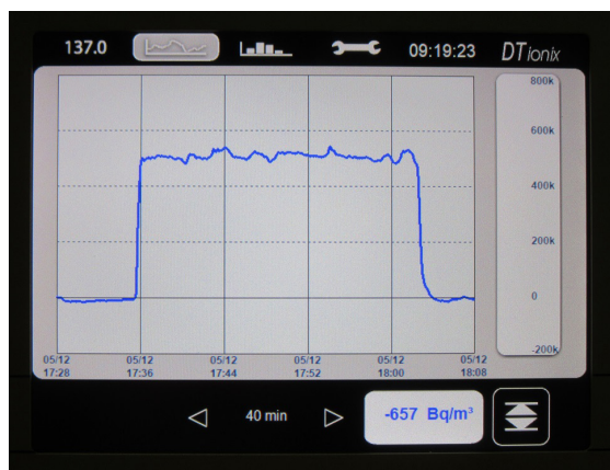
Injection of 500 kBq/m 3 (13.5 \mu Ci/m 3 ) in a C IONIX 3 - BMM
