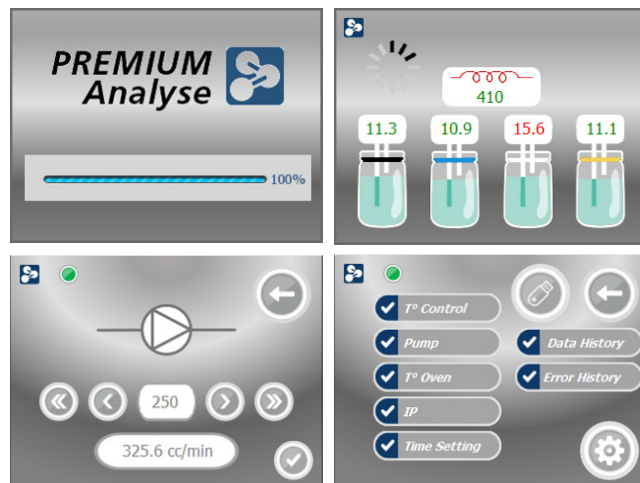
Software interface
